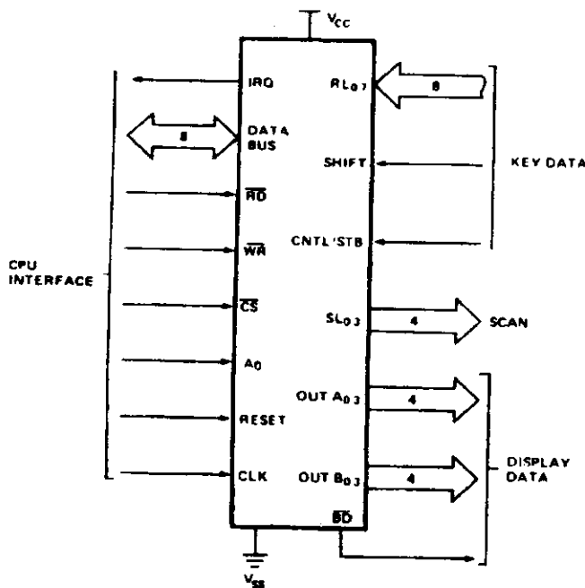
Figure 1. Logic Symbol
