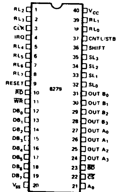
Figure 2. Pin Configuration
